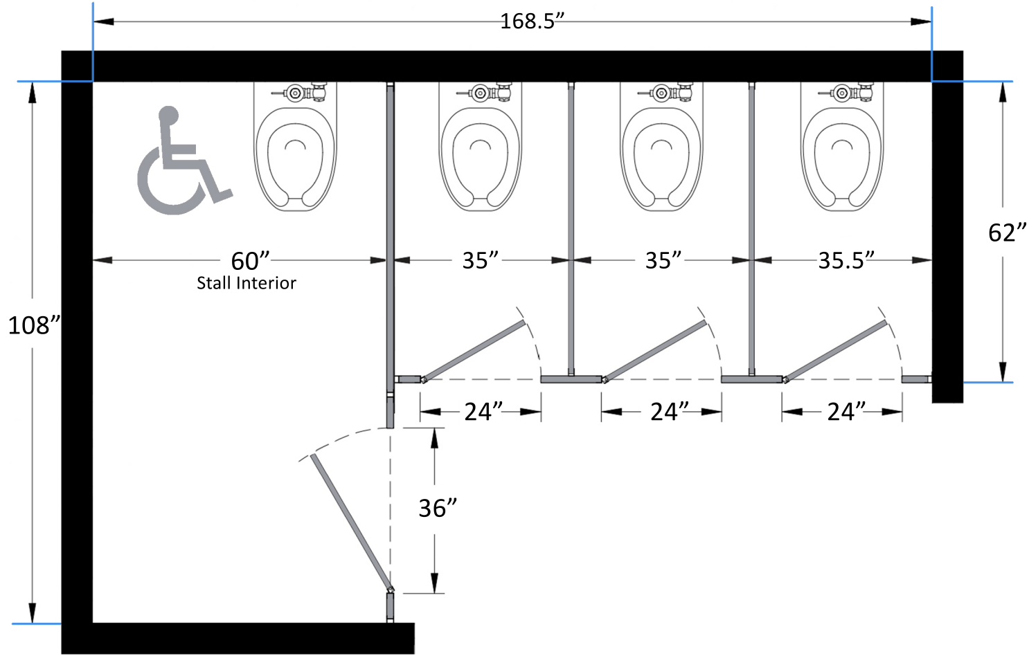
Bathroom Partitions - 4 Stall Alcove Left Hand ADA SKU: AL4LADA Standard Dimensions
